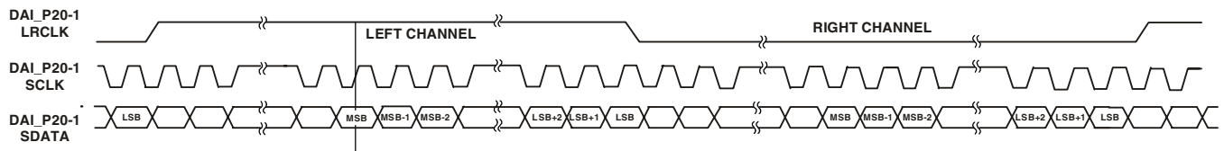
Figure 26. Right-Justified Mode
