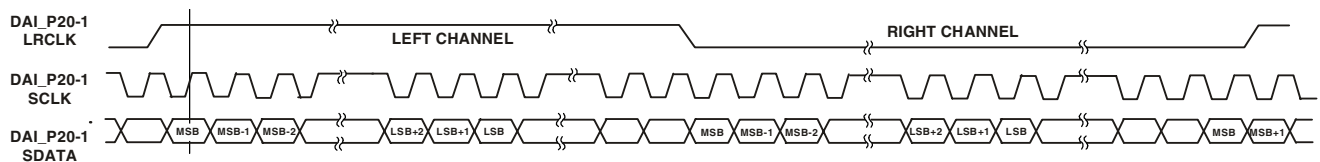
Figure 28. Left-Justified Mode
